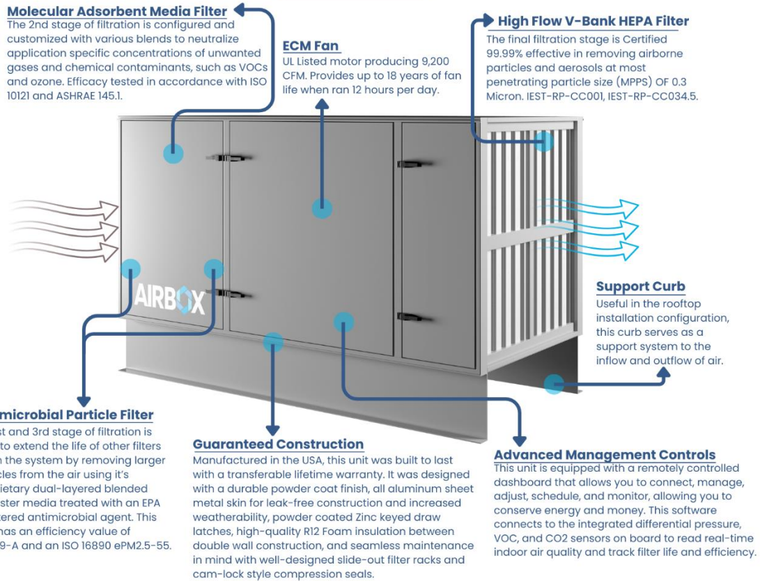
VORTEX SECTION VIEW
