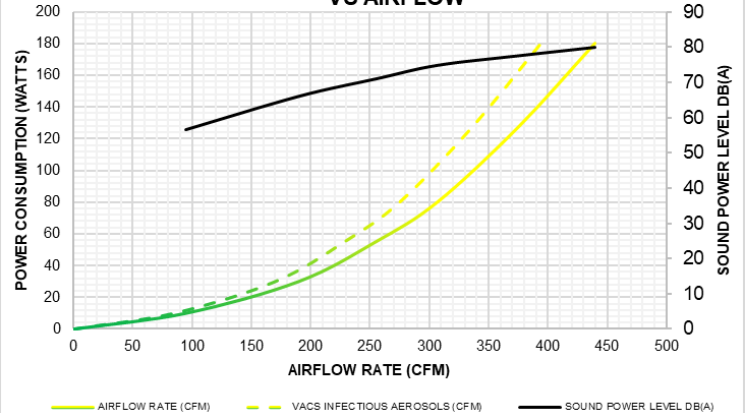
POWER CONSUMPTION AND SOUND POWER LEVEL VS AIRFLOW
